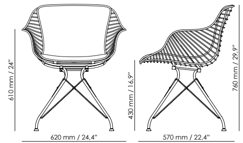
OD11-43 Seating height: 430 mm / 16,9"
