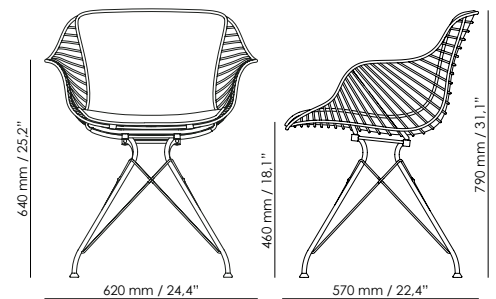
OD11-46 Seating height: 460 mm / 18,1"
